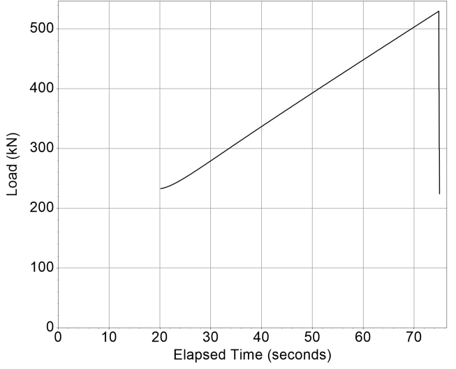
Specimen Load
