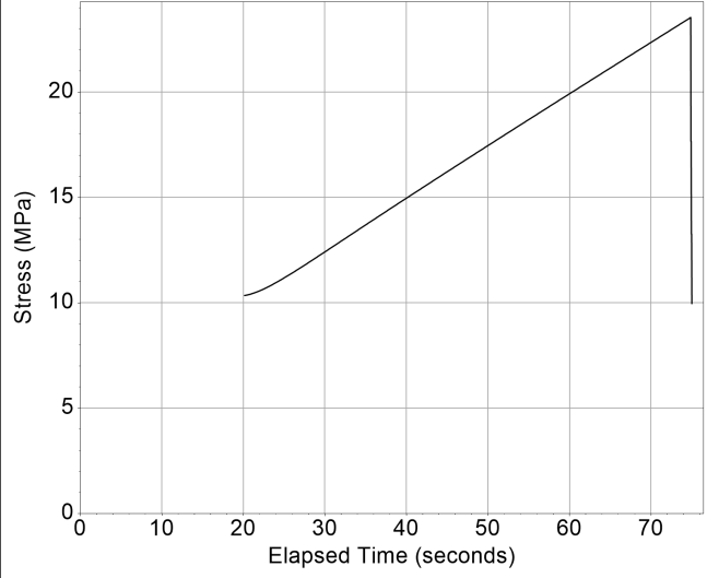
Specimen Stress
